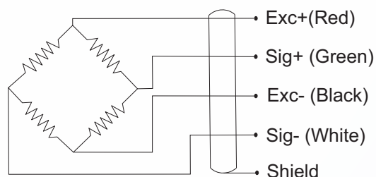
Wiring Diagram
